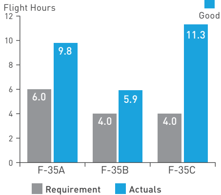
Reliability: Mean Flight Hour Between Failure
