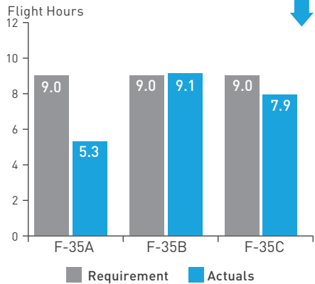
Maintainability: Maintenance Man Hour Per Flight Hour
